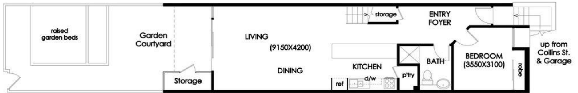
GROUND FLOOR
